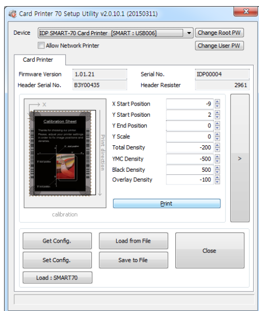
Рис. 93 CardPrinter70Setup Start
