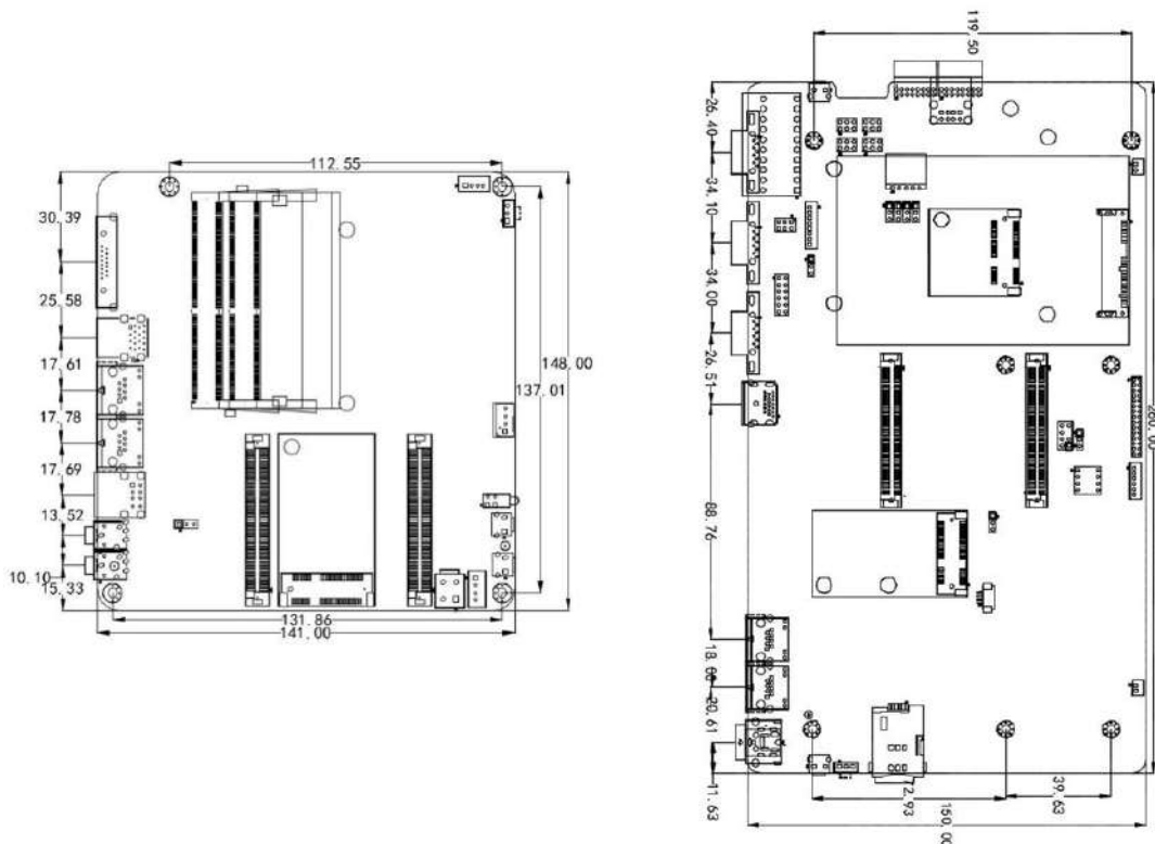
Figure 1 3.2 Main board size diagram
