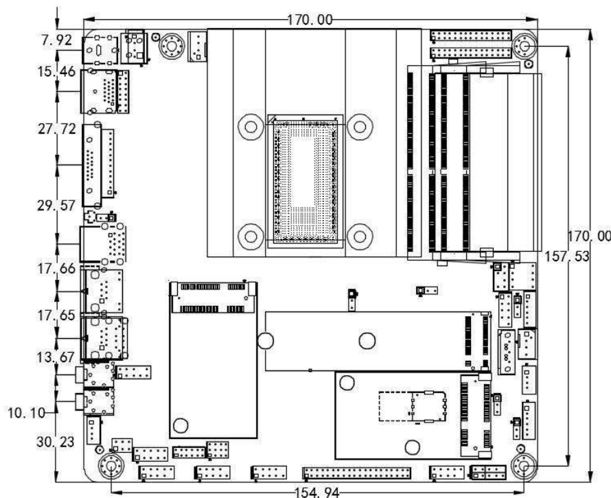
Figure 1 3.2 Main board size diagram
