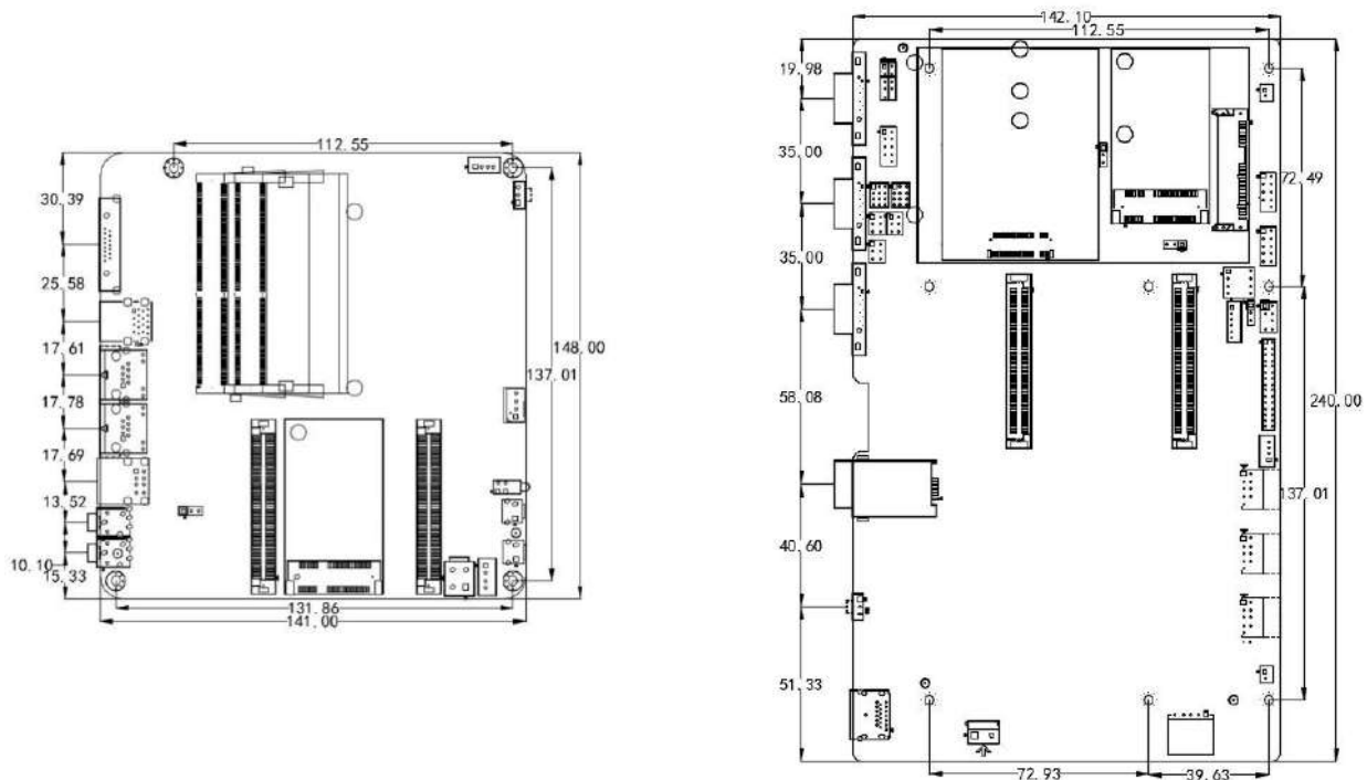
Figure 1 3.2 Main board size diagram
